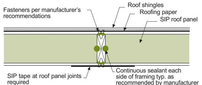
DETAIL 1.2: SIP ROOF – DIMENSIONAL LUMBER SINGLE SPLINE JOINT 8
