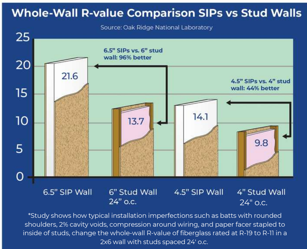
FIGURE 1.4: INSULATION COMPARISON OF SIPs TO DIMENSIONALLY FRAMED WALLS AND INSTALLATION QUALITY EFFECTS
