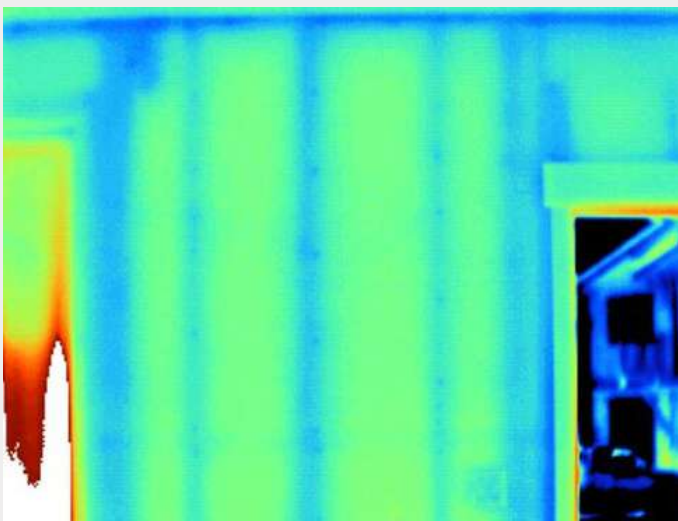
IMAGE 1.5: DIMENSIONALLY FRAMED WALL WITH THERMAL BRIDGING AT STUDS (IN BLUE)
