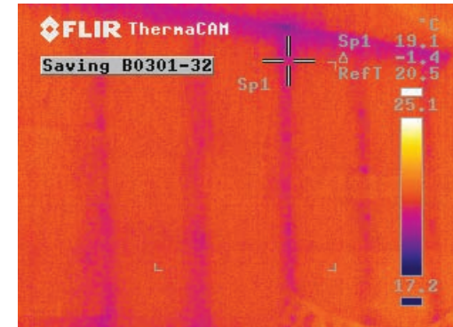
Thermal imaging of wood-framed wall shows heat escaping along studs.
